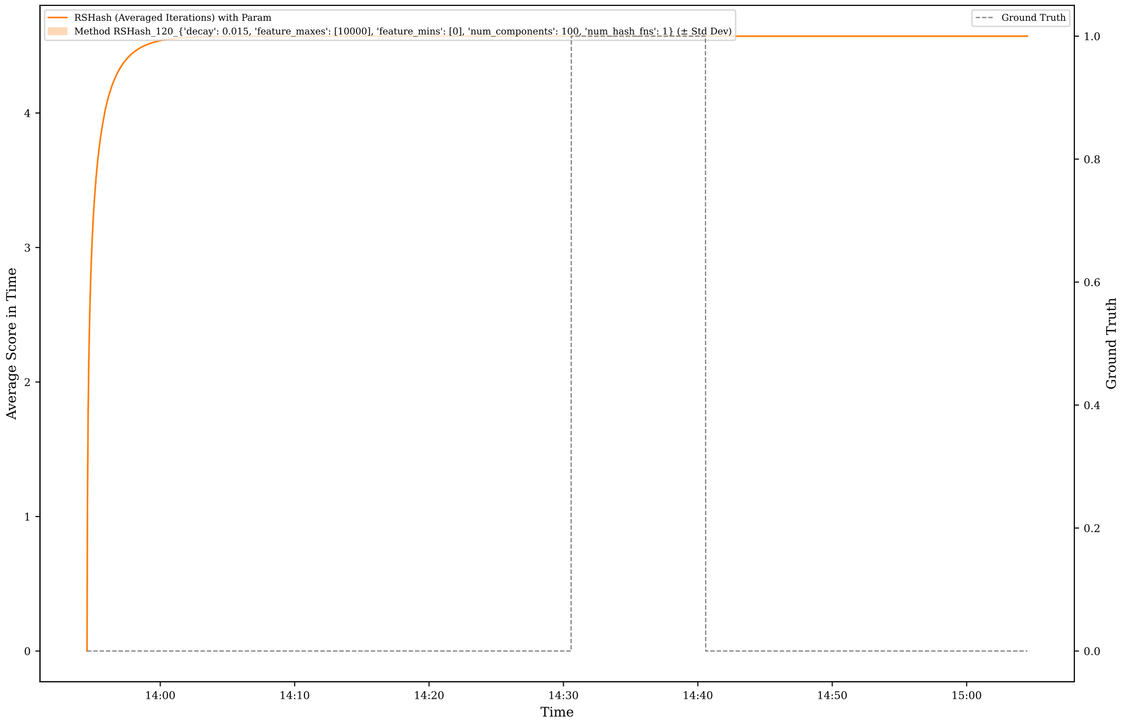
Method RSHash Score for Scenario A9
